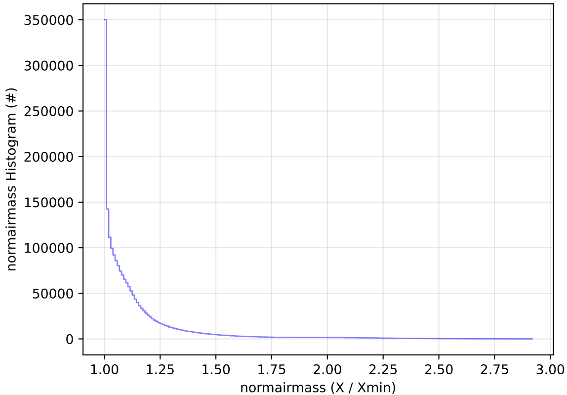
ddf_acor_sf30_lsf40_lsr10_v3.4_10yrs WFD all bands: normairmass Histogram
