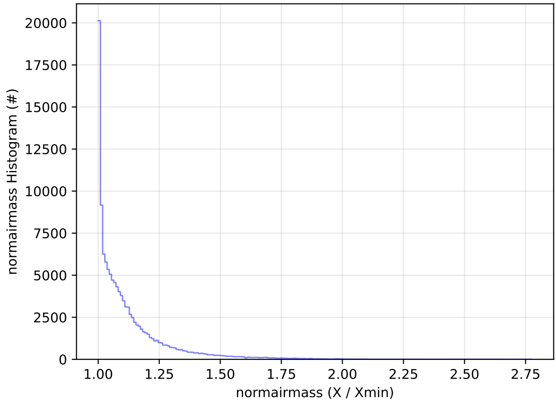
ddf_acor_sf30_lsf40_lsr10_v3.4_10yrs All sky u band: normairmass Histogram
