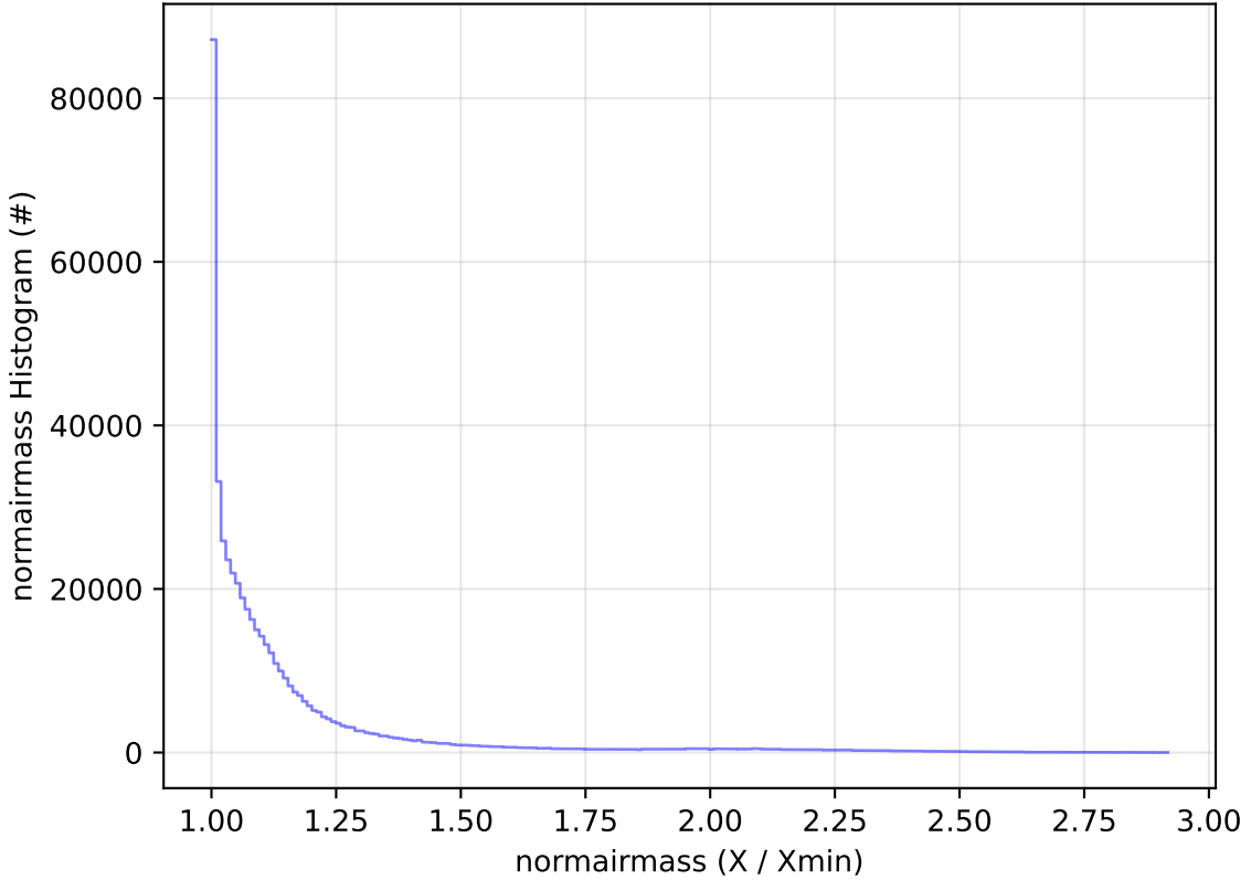
ddf_acor_sf30_lsf40_lsr10_v3.4_10yrs All sky i band: normairmass Histogram
