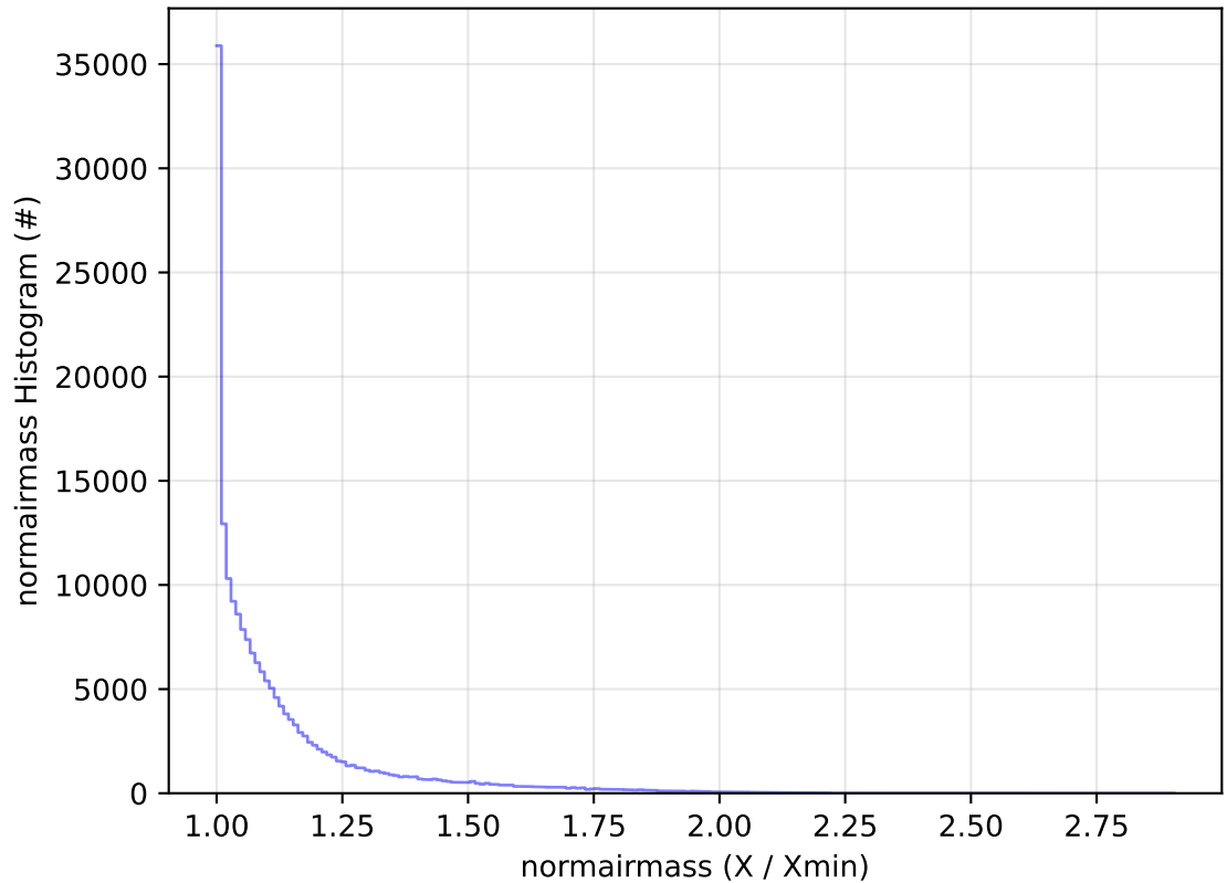
ddf_acor_sf30_lsf40_lsr10_v3.4_10yrs All sky g band: normairmass Histogram
