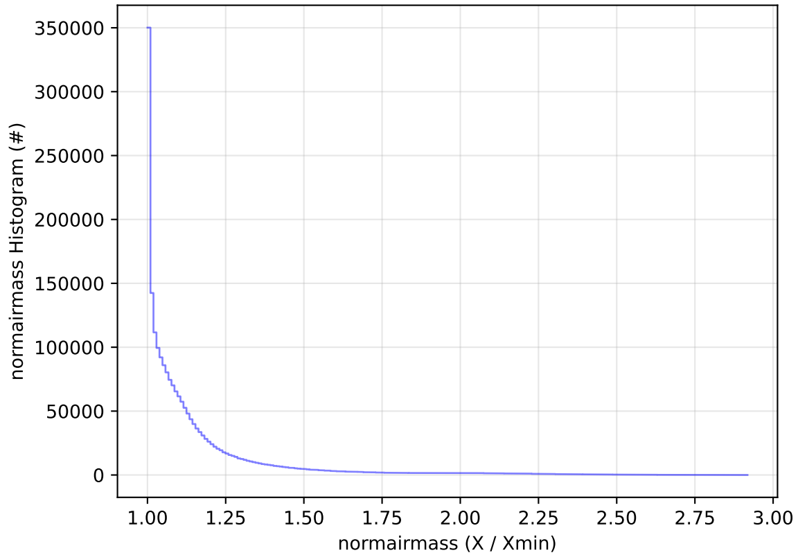
ddf_acor_sf30_lsf40_lsr10_v3.4_10yrs All sky all bands: normairmass Histogram
