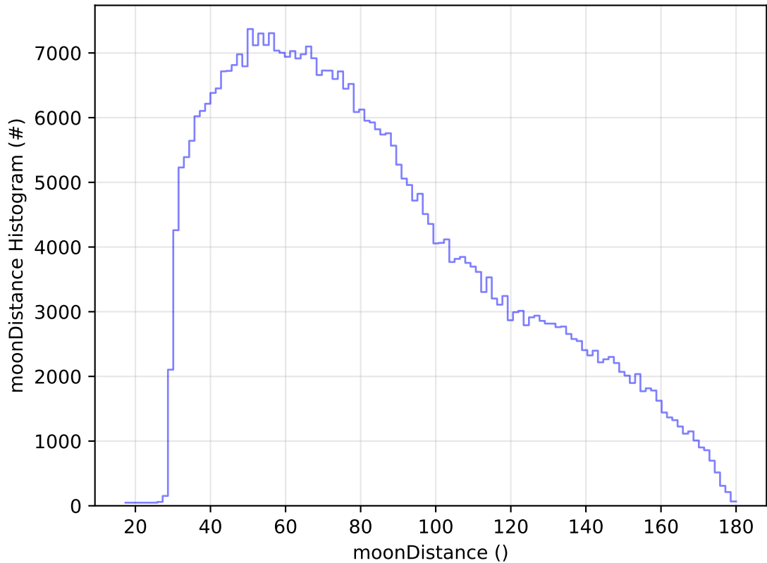
ddf_acor_sf30_Isf40_Isr10_v3.4_10yrs WFD z band: moonDistance Histogram
