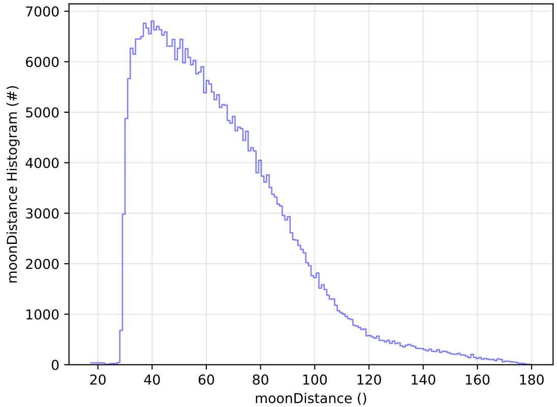
ddf_acor_sf30_Isf40_Isr10_v3.4_10yrs WFD y band: moonDistance Histogram
