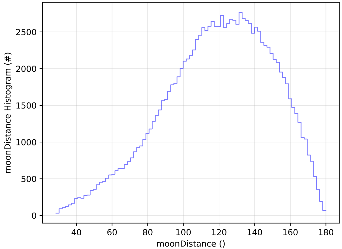
ddf_acor_sf30_lsf40_lsr10_v3.4_10yrs WFD u band: moonDistance Histogram
