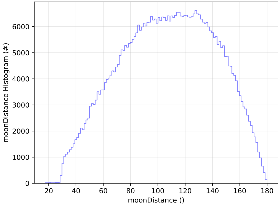
ddf_acor_sf30_lsf40_lsr10_v3.4_10yrs WFD r band: moonDistance Histogram
