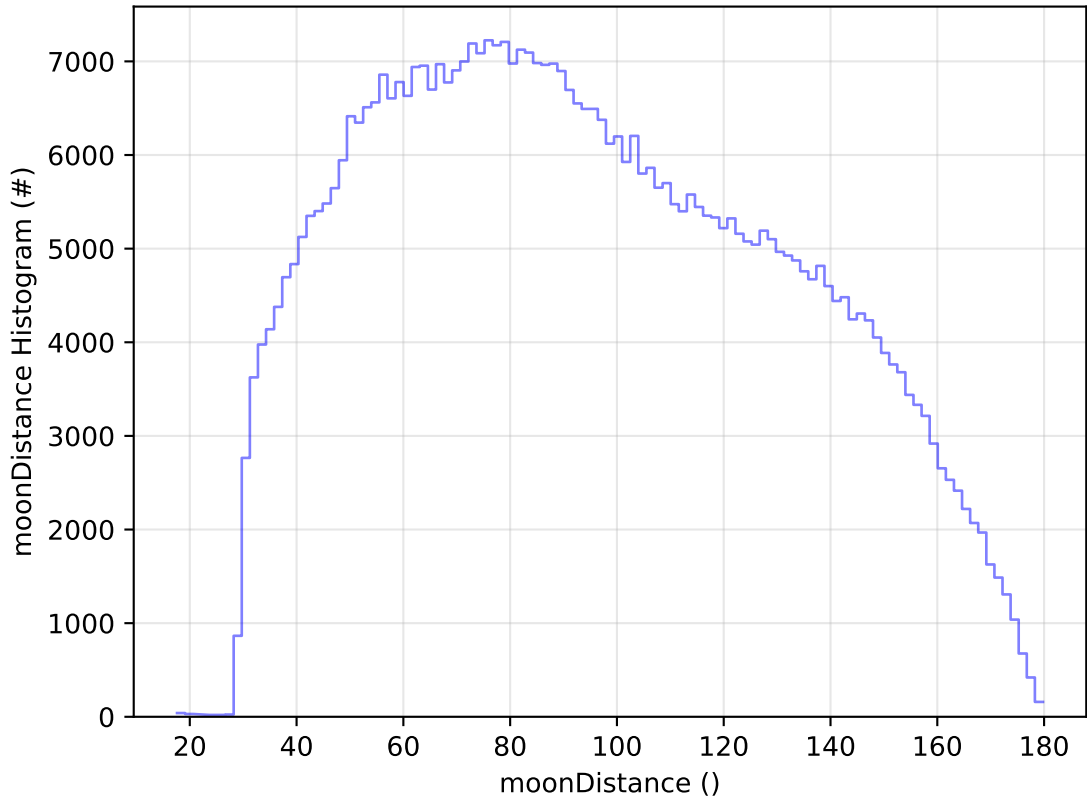
ddf_acor_sf30_lsf40_lsr10_v3.4_10yrs WFD i band: moonDistance Histogram
