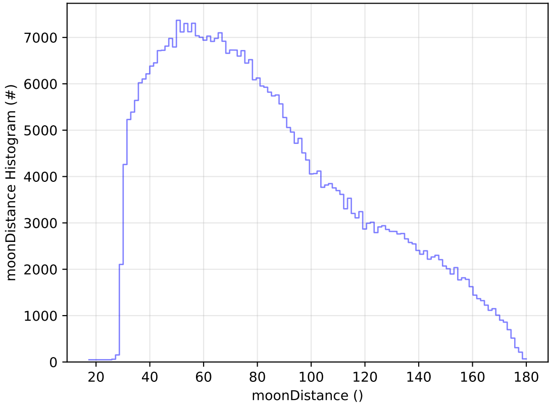
ddf_acor_sf30_lsf40_lsr10_v3.4_10yrs All sky z band: moonDistance Histogram
