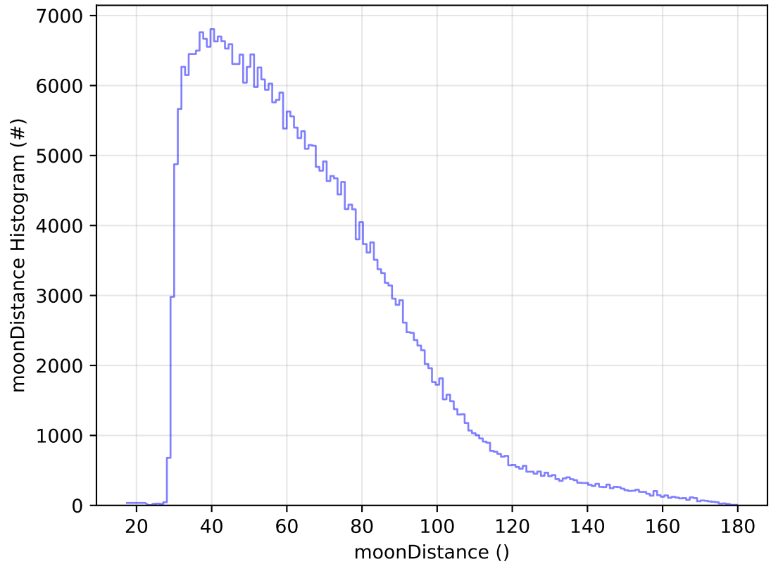
ddf_acor_sf30_lsf40_lsr10_v3.4_10yrs All sky y band: moonDistance Histogram
