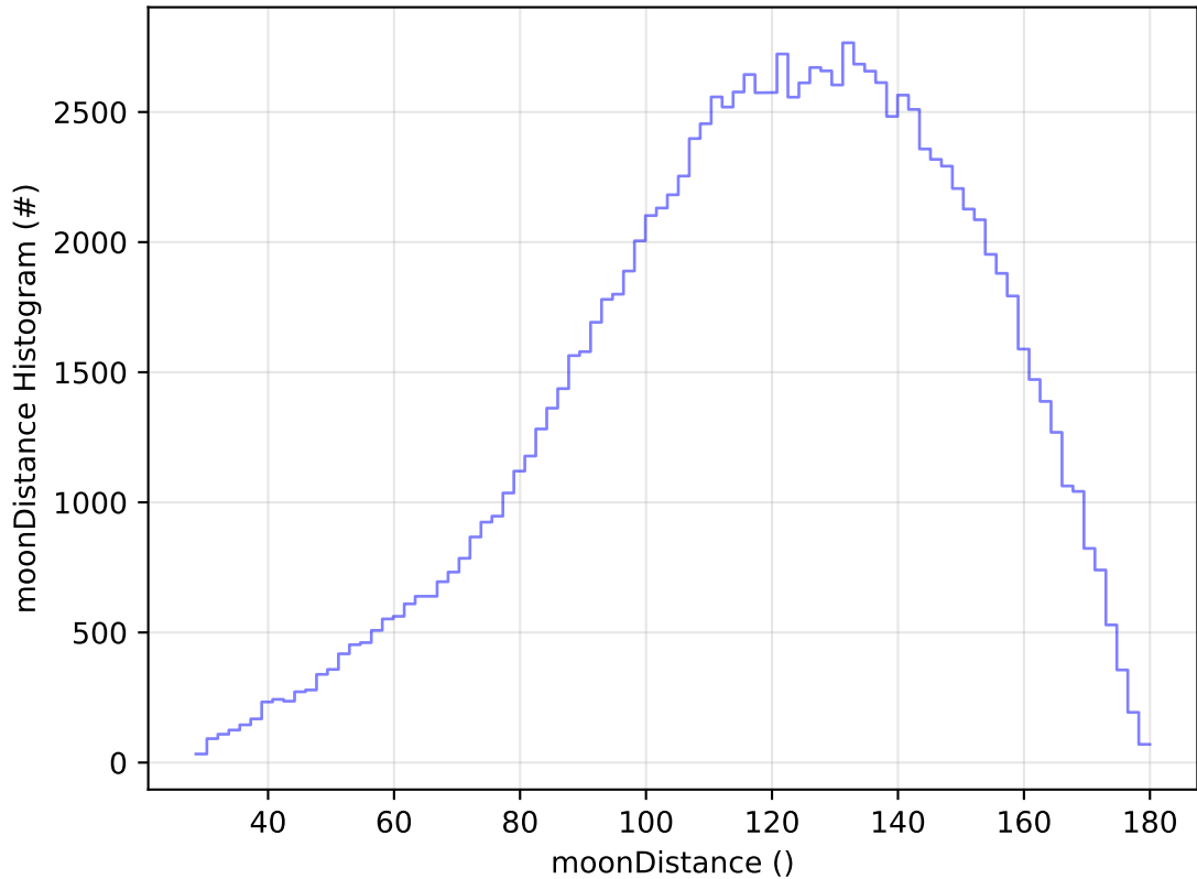
ddf_acor_sf30_lsf40_lsr10_v3.4_10yrs All sky u band: moonDistance Histogram
