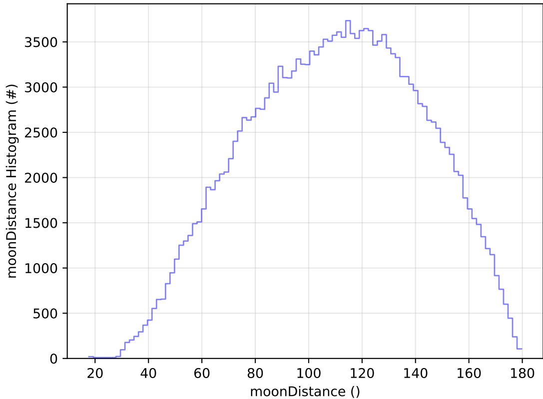
ddf_acor_sf30_lsf40_lsr10_v3.4_10yrs All sky g band: moonDistance Histogram
