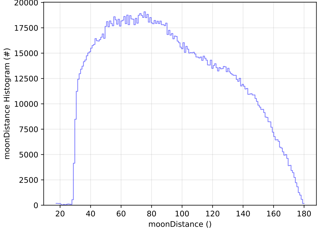
ddf_acor_sf30_lsf40_lsr10_v3.4_10yrs All sky all bands: moonDistance Histogram
