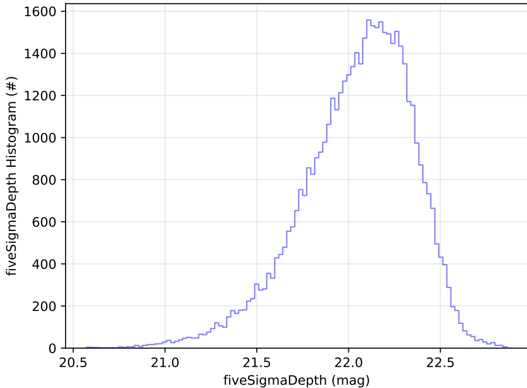
ddf_acor_sf30_lsf40_lsr10_v3.4_10yrs Yr 1 y band: fiveSigmaDepth Histogram
