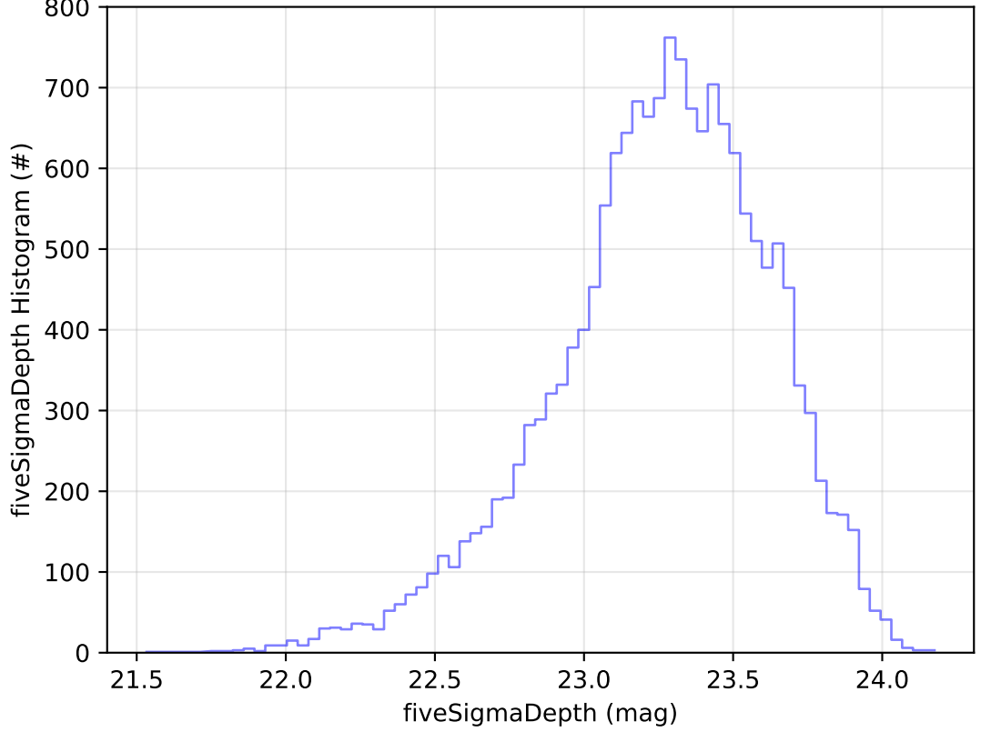
ddf_acor_sf30_lsf40_lsr10_v3.4_10yrs Yr 1 u band: fiveSigmaDepth Histogram
