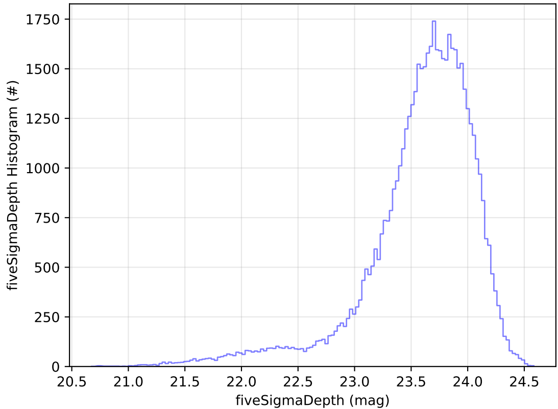
ddf_acor_sf30_lsf40_lsr10_v3.4_10yrs Yr 1 i band: fiveSigmaDepth Histogram
