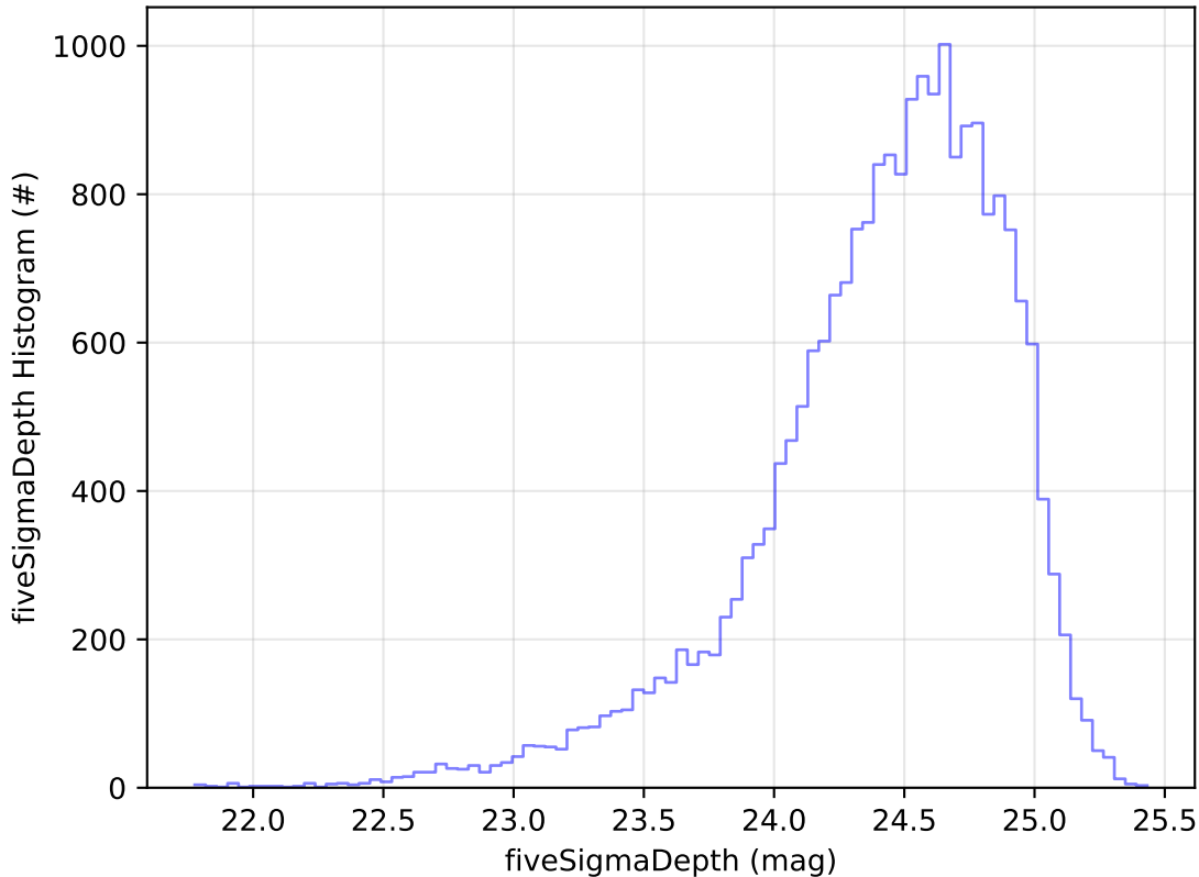
ddf_acor_sf30_lsf40_lsr10_v3.4_10yrs Yr 1 g band: fiveSigmaDepth Histogram
