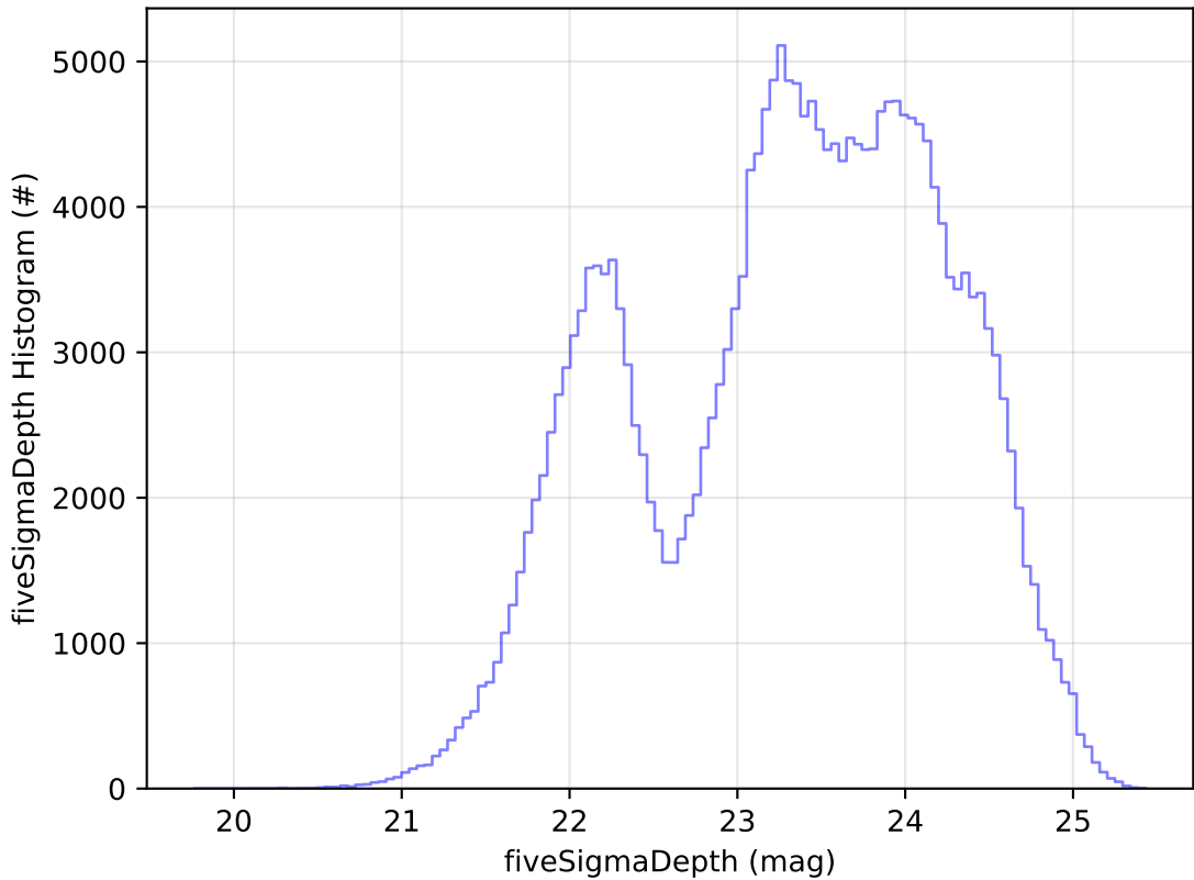
ddf_acor_sf30_lsf40_lsr10_v3.4_10yrs Yr 1 all bands: fiveSigmaDepth Histogram
