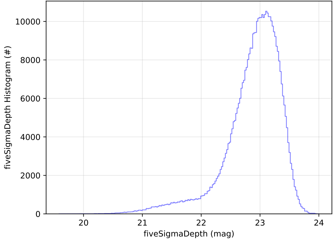
ddf_acor_sf30_lsf40_lsr10_v3.4_10yrs WFD z band: fiveSigmaDepth Histogram
