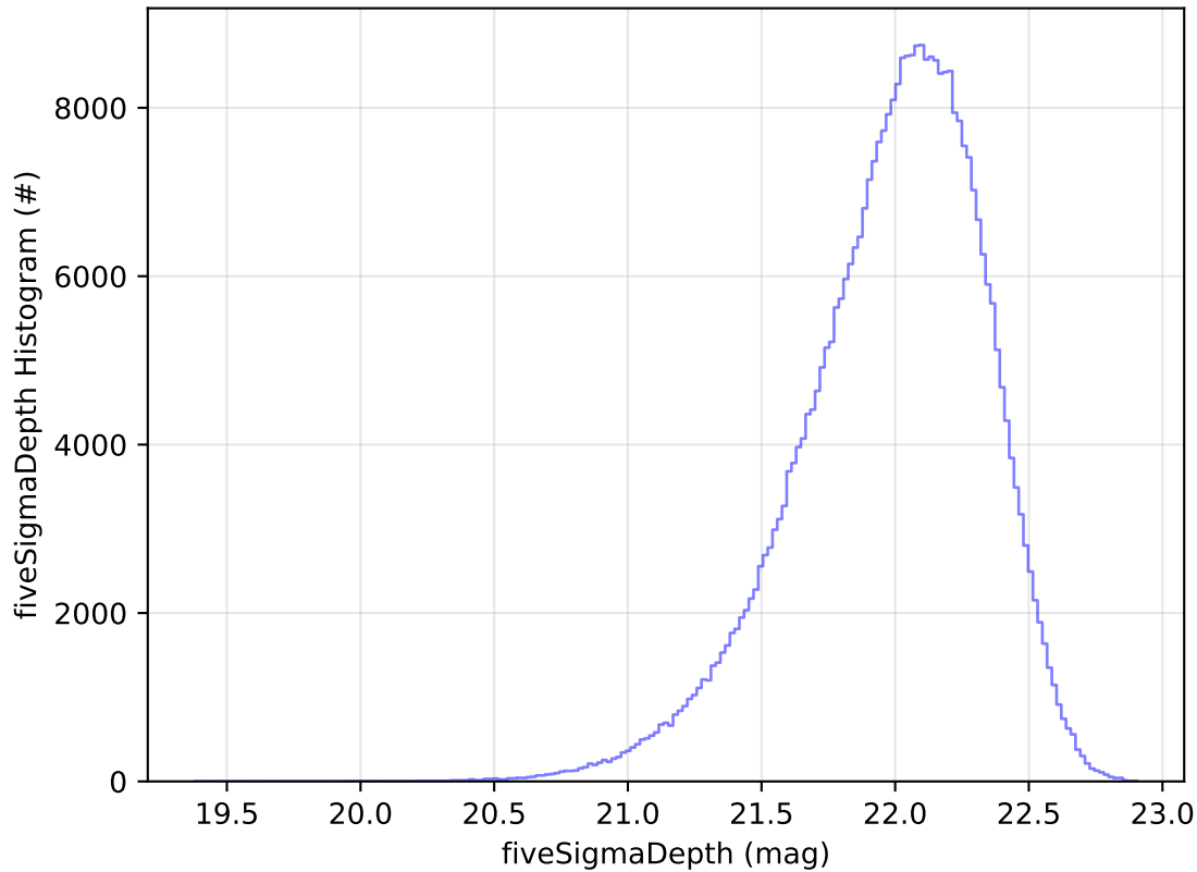
ddf_acor_sf30_lsf40_lsr10_v3.4_10yrs WFD y band: fiveSigmaDepth Histogram
