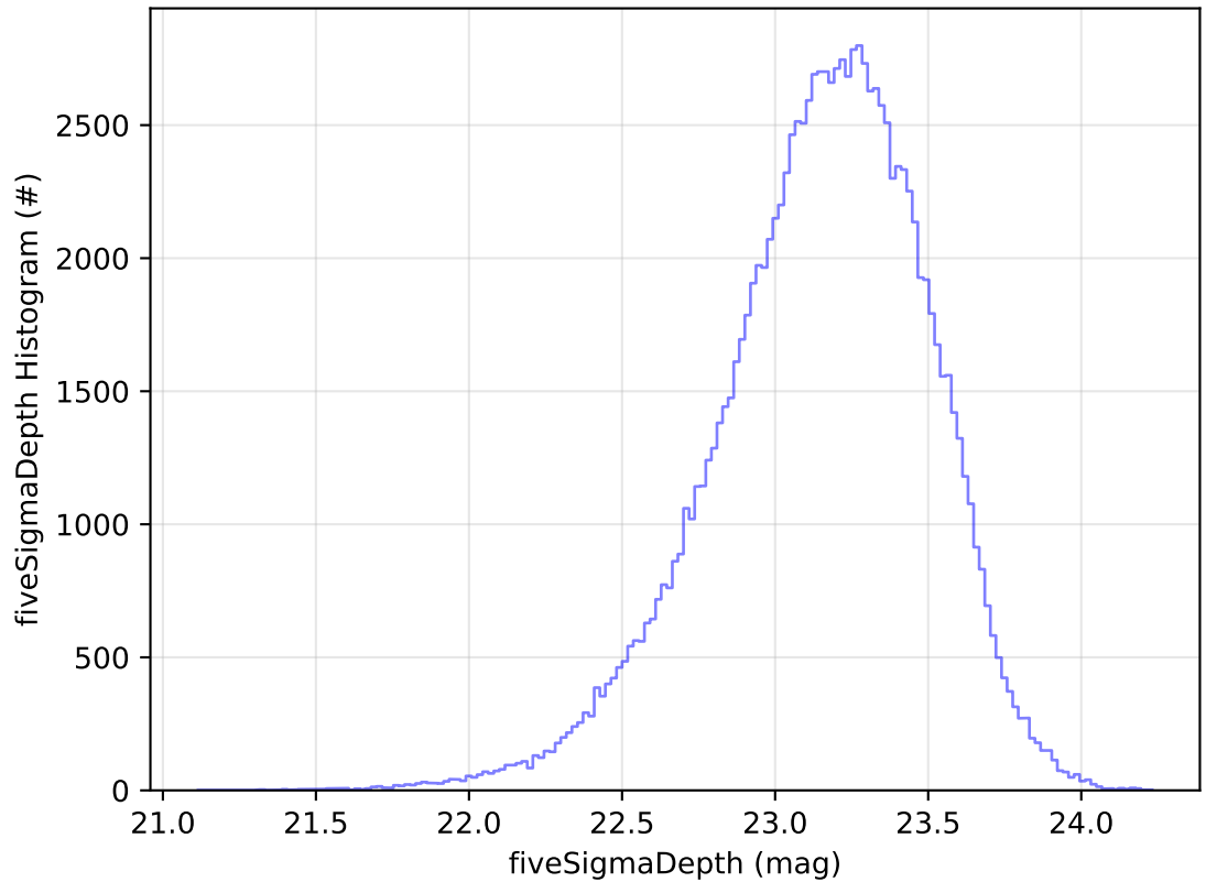
ddf_acor_sf30_lsf40_lsr10_v3.4_10yrs WFD u band: fiveSigmaDepth Histogram
