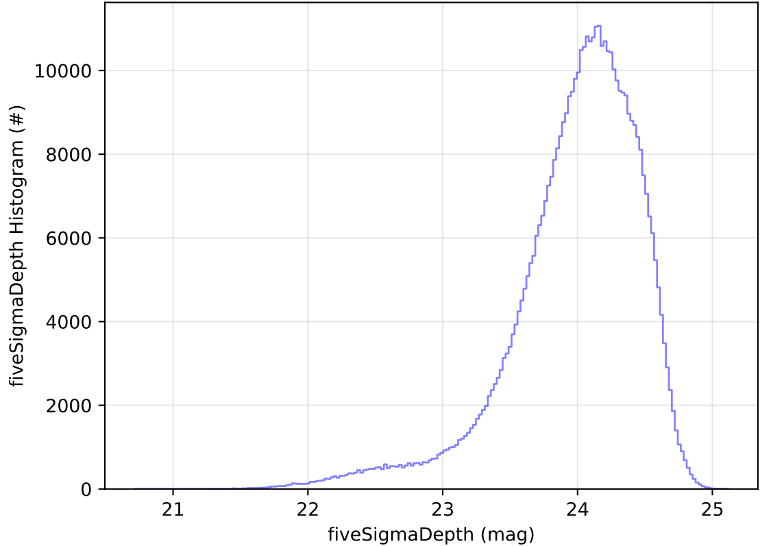
ddf_acor_sf30_lsf40_lsr10_v3.4_10yrs WFD r band: fiveSigmaDepth Histogram
