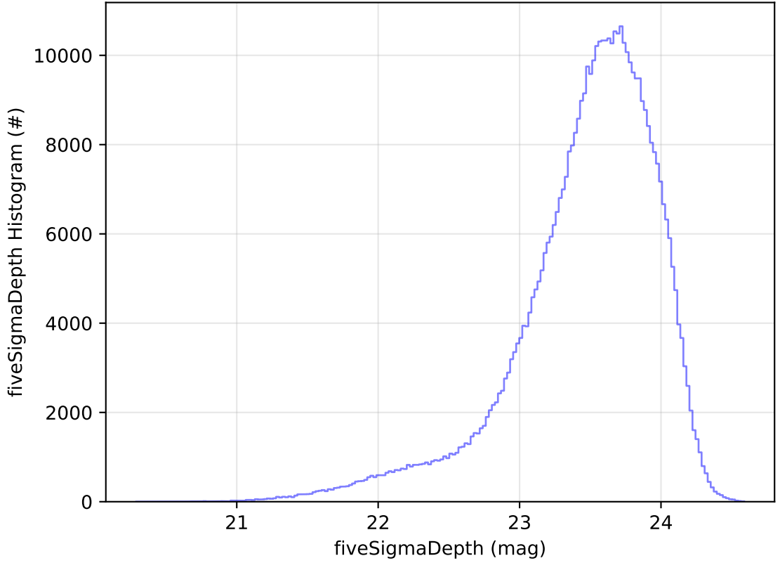
ddf_acor_sf30_lsf40_lsr10_v3.4_10yrs WFD i band: fiveSigmaDepth Histogram
