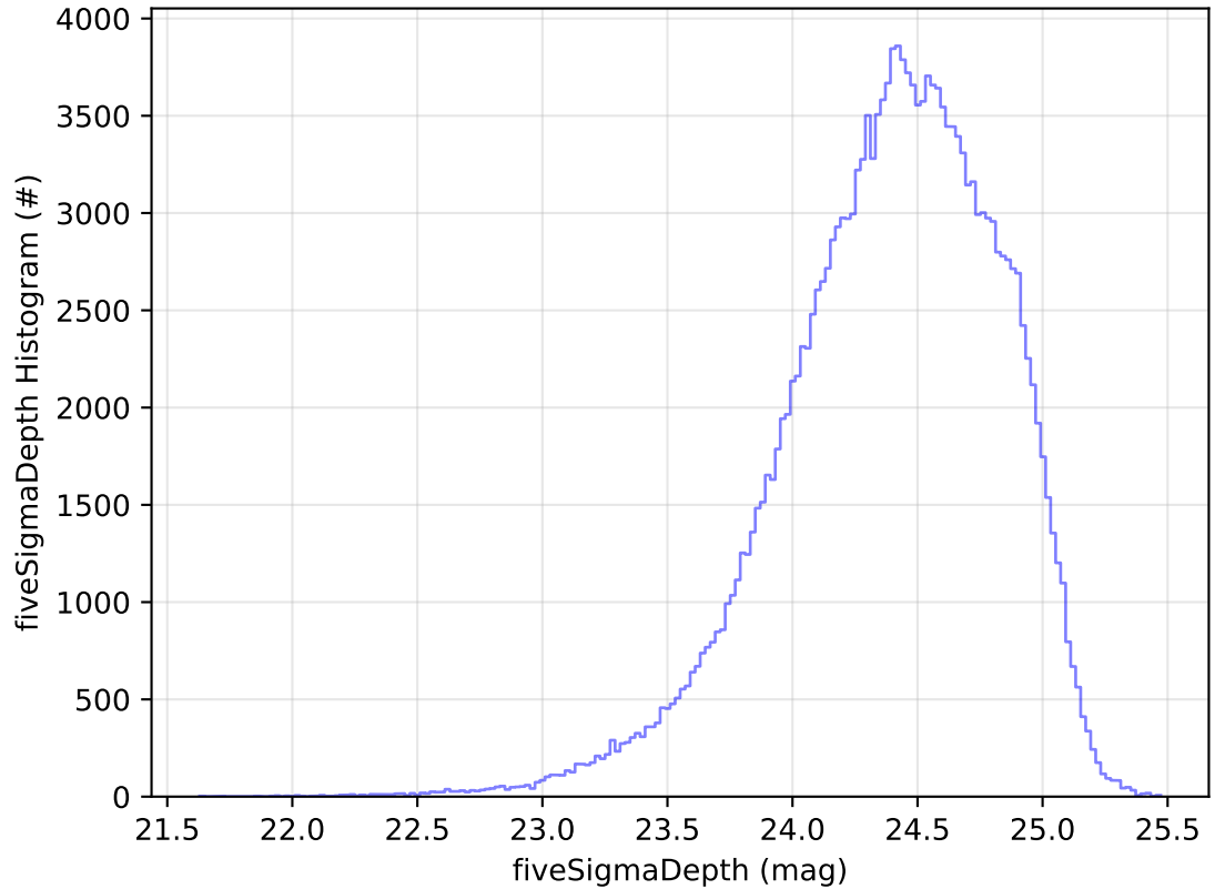
ddf_acor_sf30_lsf40_lsr10_v3.4_10yrs WFD g band: fiveSigmaDepth Histogram
