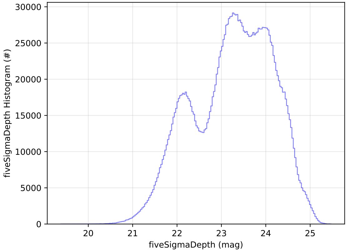
ddf_acor_sf30_lsf40_lsr10_v3.4_10yrs WFD all bands: fiveSigmaDepth Histogram
