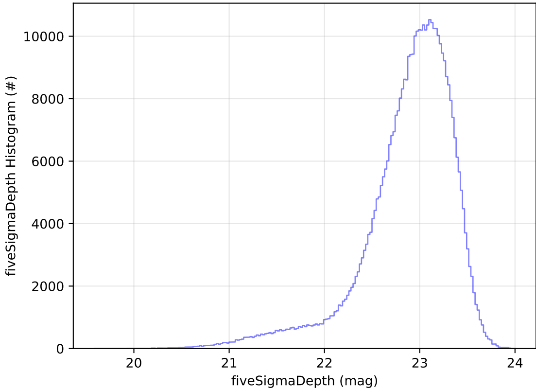
ddf_acor_sf30_lsf40_lsr10_v3.4_10yrs All sky z band: fiveSigmaDepth Histogram
