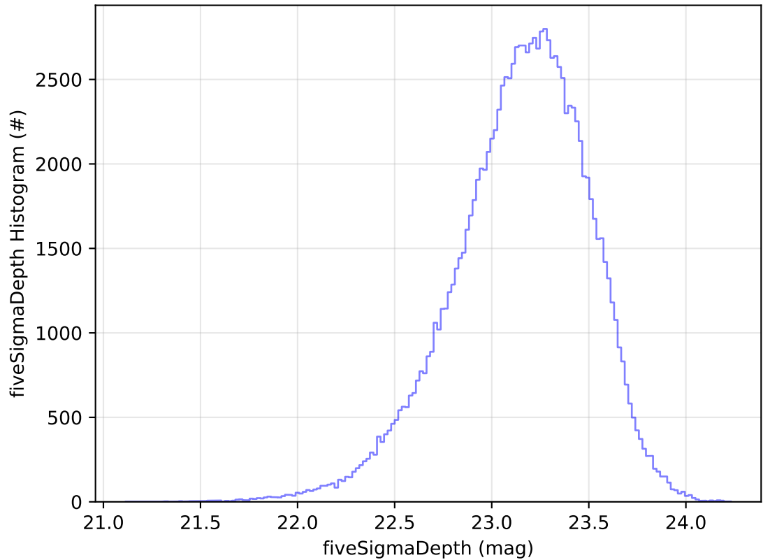
ddf_acor_sf30_lsf40_lsr10_v3.4_10yrs All sky u band: fiveSigmaDepth Histogram
