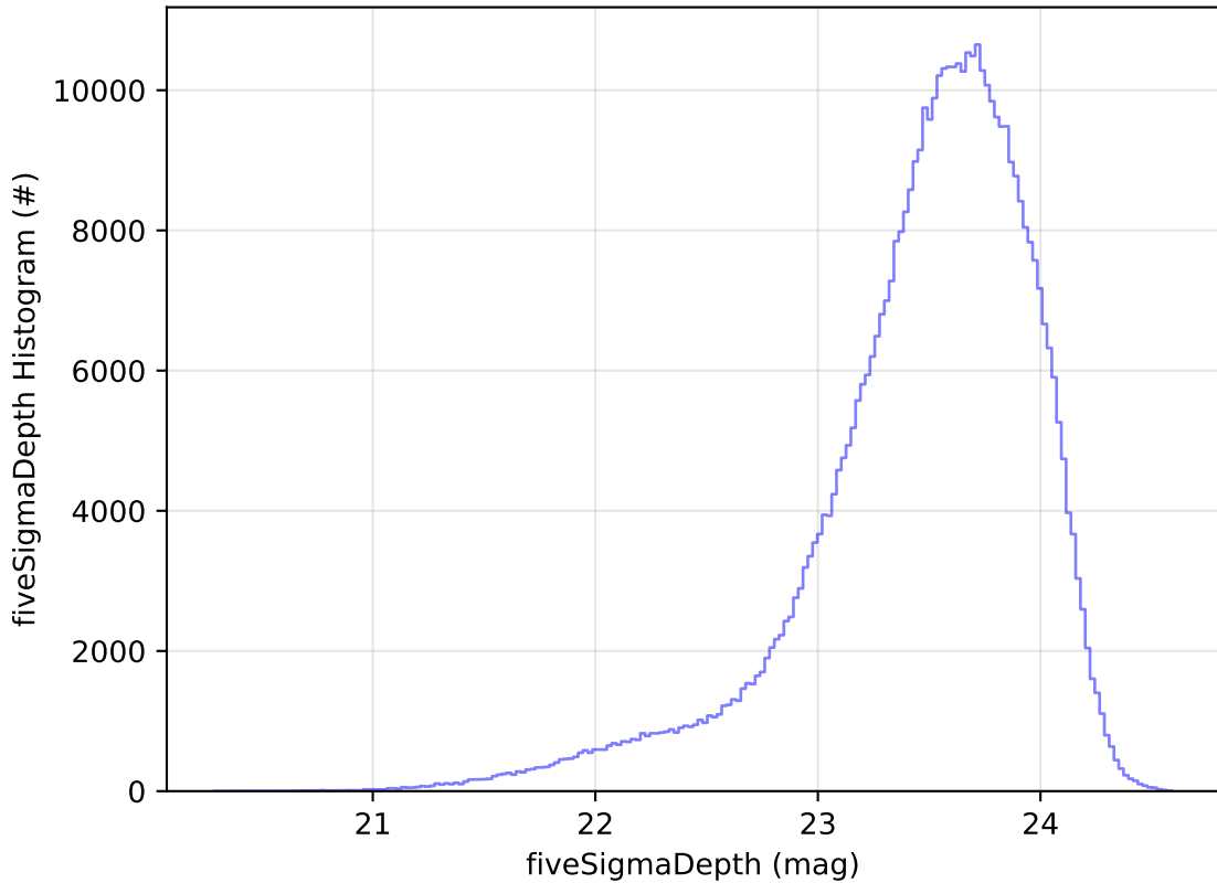
ddf_acor_sf30_lsf40_lsr10_v3.4_10yrs All sky i band: fiveSigmaDepth Histogram
