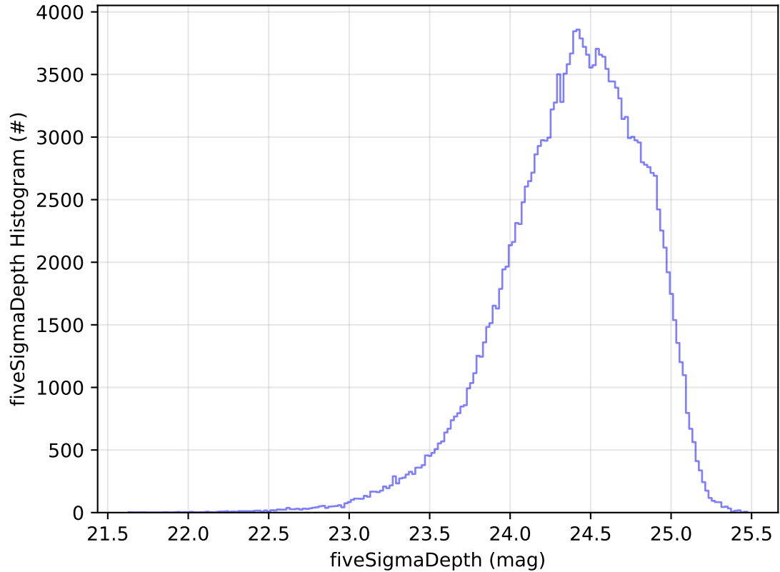
ddf_acor_sf30_lsf40_lsr10_v3.4_10yrs All sky g band: fiveSigmaDepth Histogram
