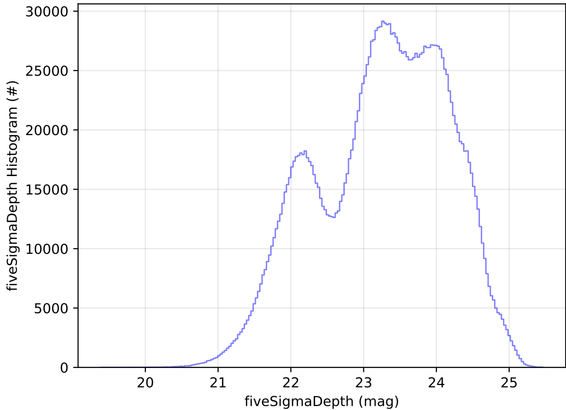
ddf_acor_sf30_lsf40_lsr10_v3.4_10yrs All sky all bands: fiveSigmaDepth Histogram
