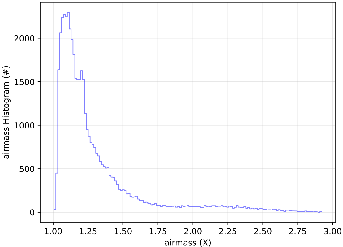
ddf_acor_sf30_lsf40_lsr10_v3.4_10yrs Yr 1 z band: airmass Histogram
