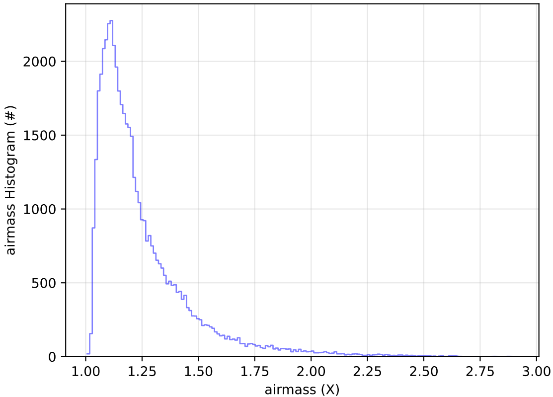
ddf_acor_sf30_lsf40_lsr10_v3.4_10yrs Yr 1 y band: airmass Histogram
