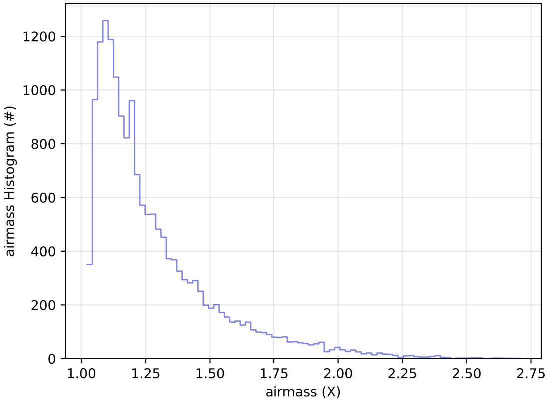
ddf_acor_sf30_lsf40_lsr10_v3.4_10yrs Yr 1 u band: airmass Histogram
