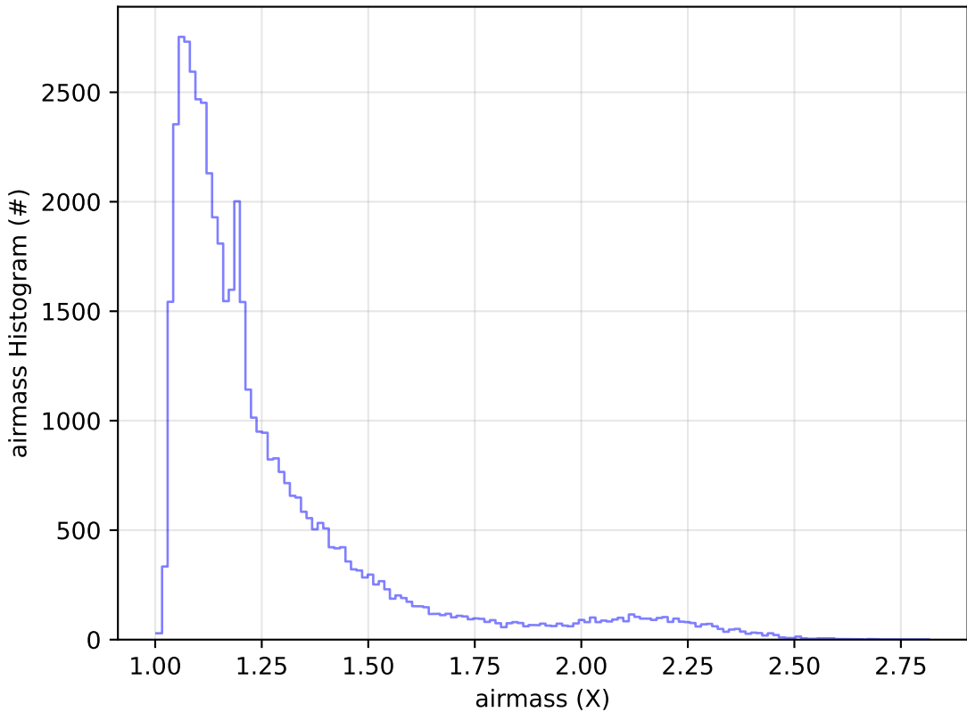
ddf_acor_sf30_Isf40_Isr10_v3.4_10yrs Yr 1 r band: airmass Histogram
