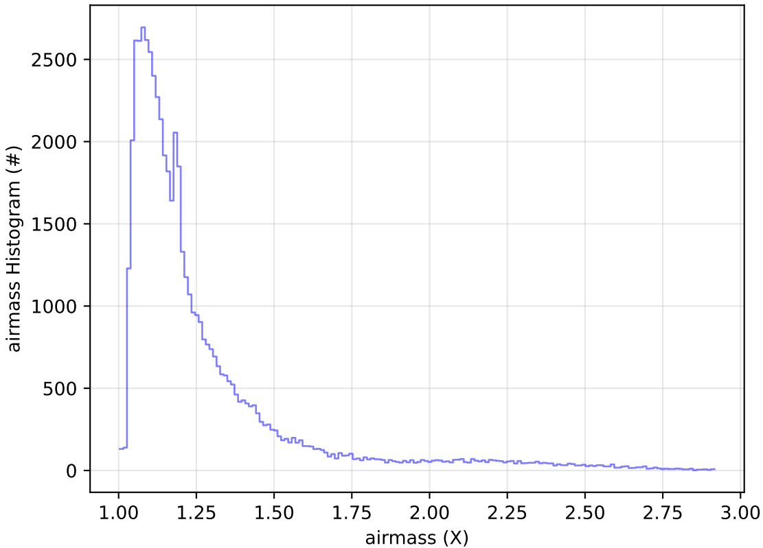
ddf_acor_sf30_lsf40_lsr10_v3.4_10yrs Yr 1 i band: airmass Histogram
