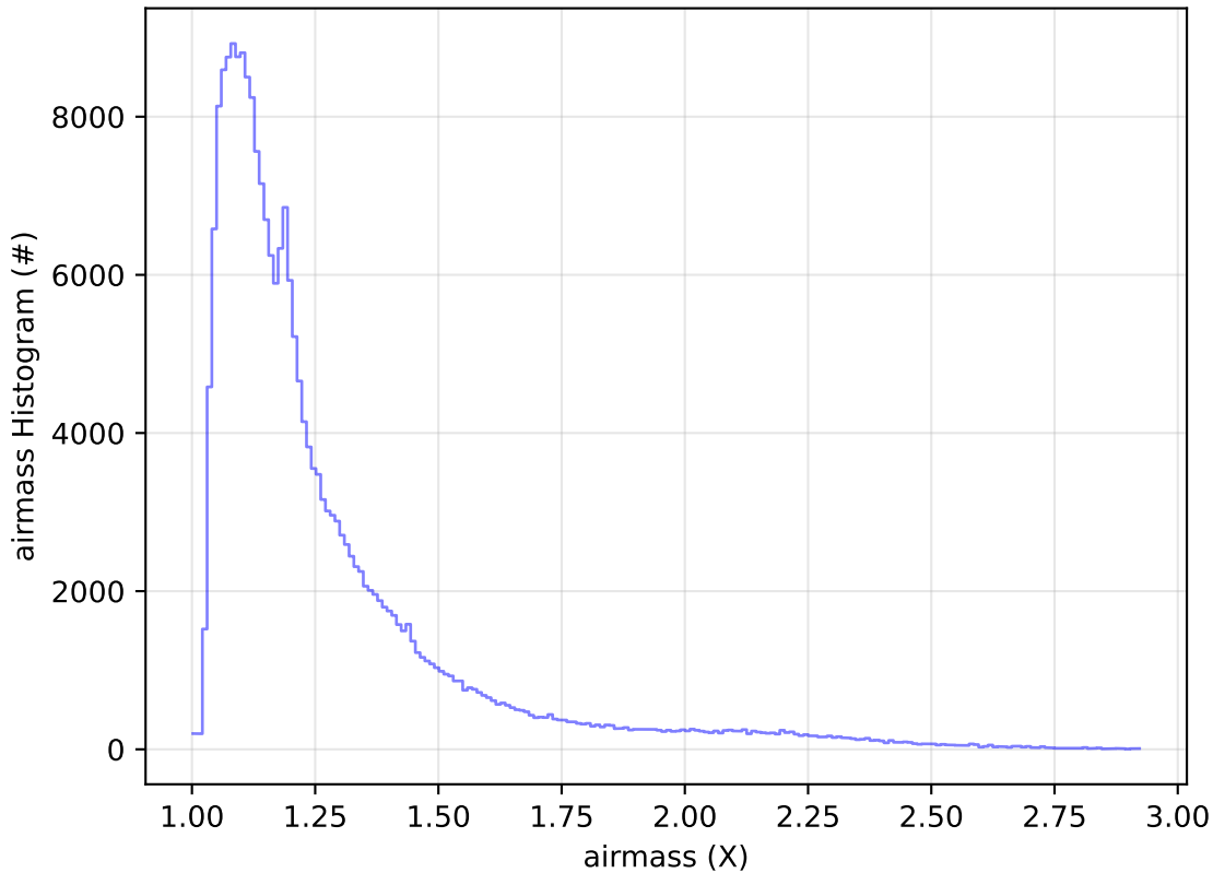
ddf_acor_sf30_lsf40_lsr10_v3.4_10yrs Yr 1 all bands: airmass Histogram
