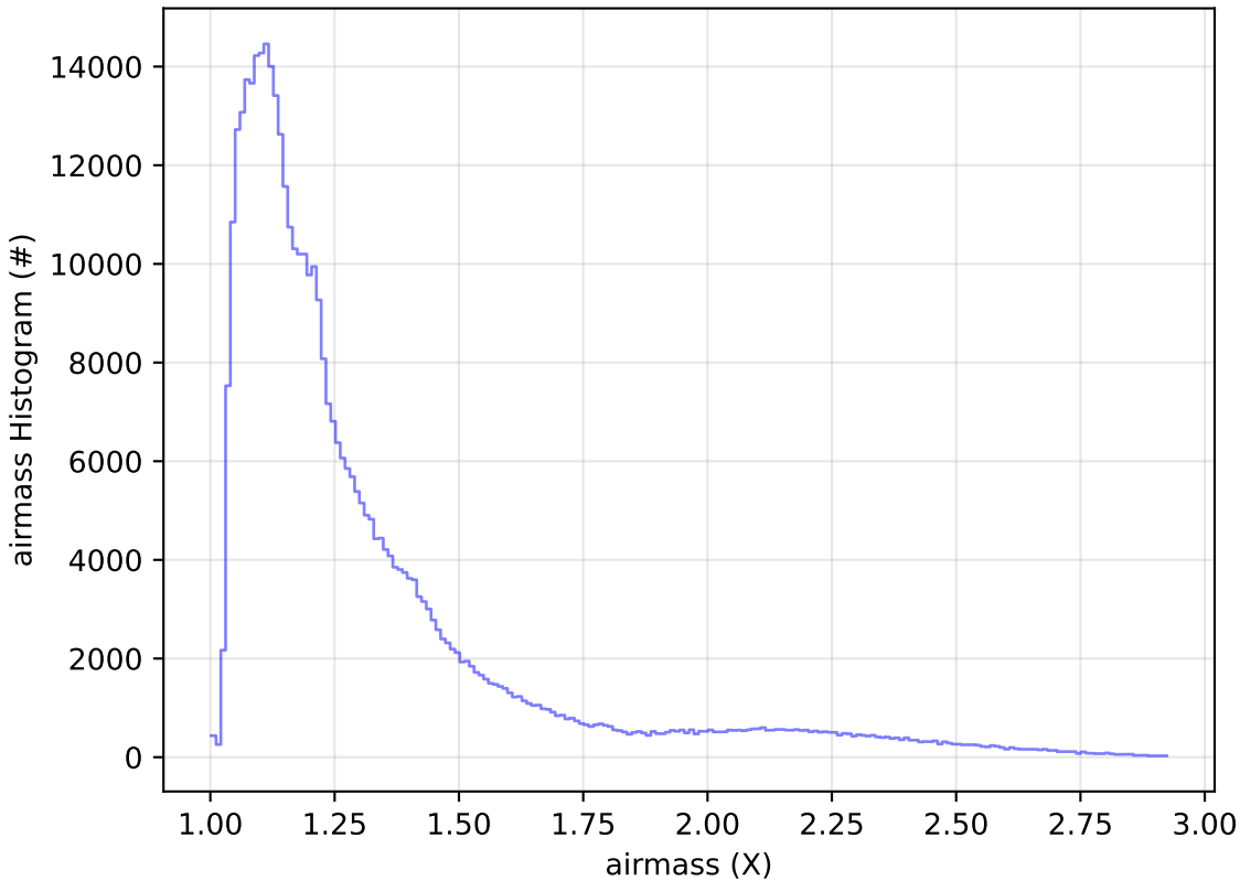
ddf_acor_sf30_lsf40_lsr10_v3.4_10yrs WFD z band: airmass Histogram
