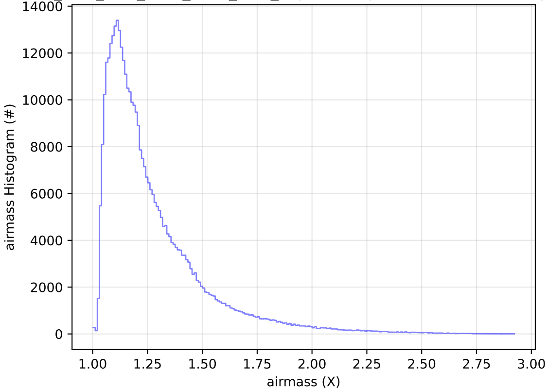
ddf_acor_sf30_lsf40_lsr10_v3.4_10yrs WFD y band: airmass Histogram
