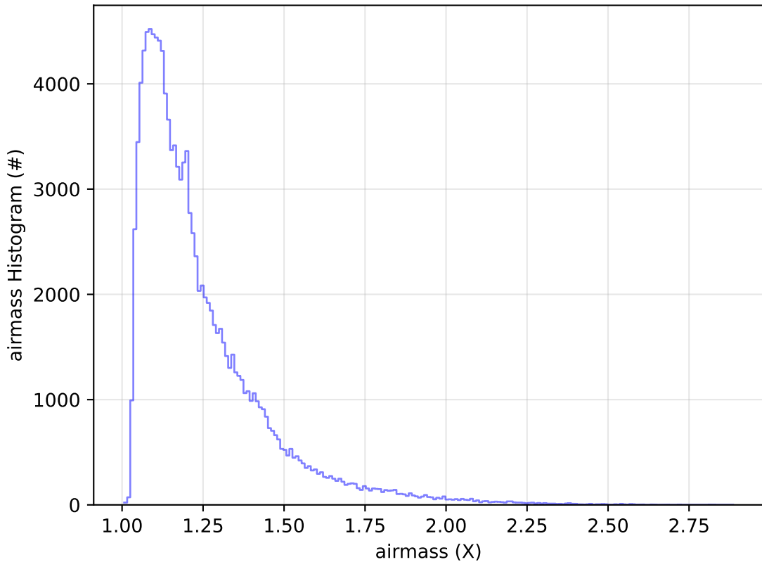
ddf_acor_sf30_lsf40_lsr10_v3.4_10yrs WFD u band: airmass Histogram
