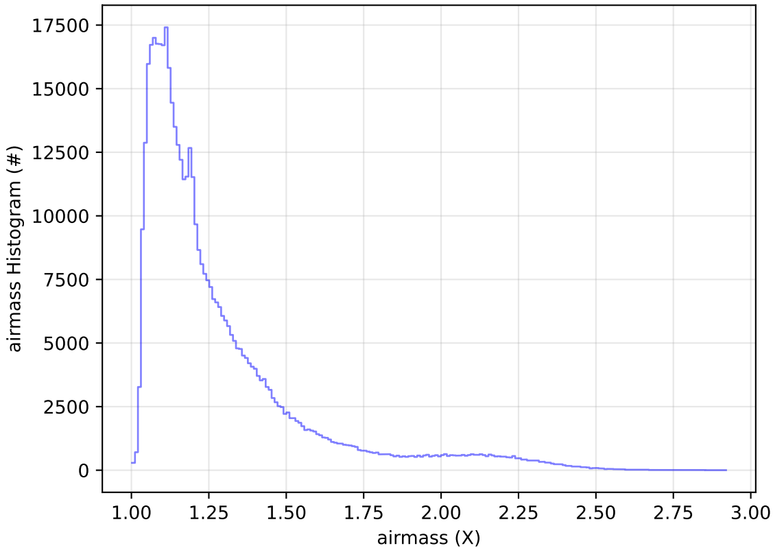
ddf_acor_sf30_Isf40_Isr10_v3.4_10yrs WFD r band: airmass Histogram
