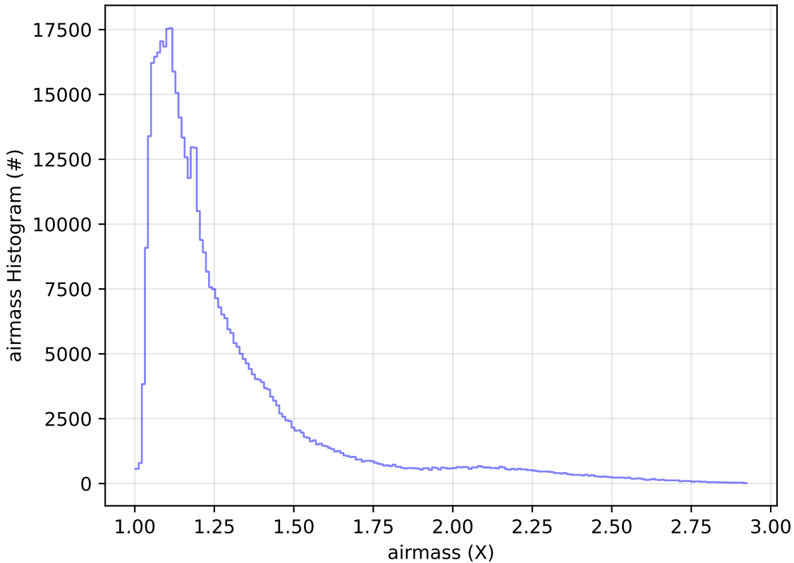
ddf_acor_sf30_lsf40_lsr10_v3.4_10yrs WFD i band: airmass Histogram
