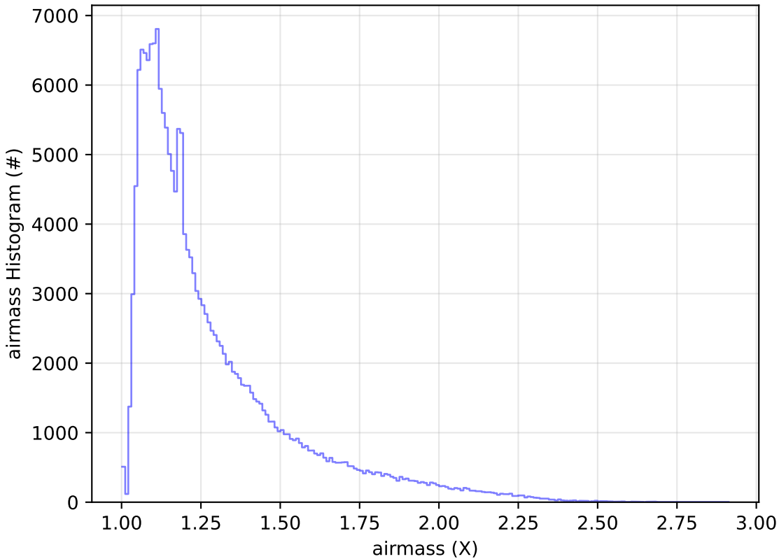
ddf_acor_sf30_lsf40_lsr10_v3.4_10yrs WFD g band: airmass Histogram
