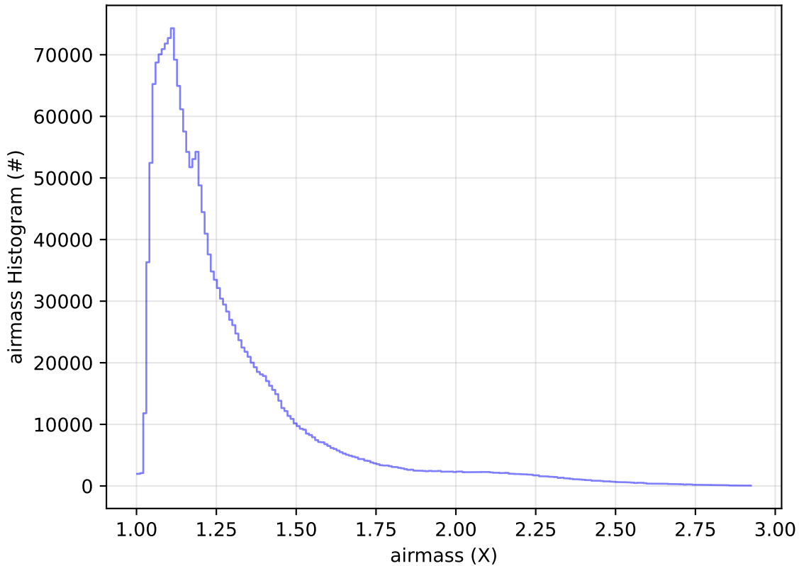
ddf_acor_sf30_lsf40_lsr10_v3.4_10yrs WFD all bands: airmass Histogram
