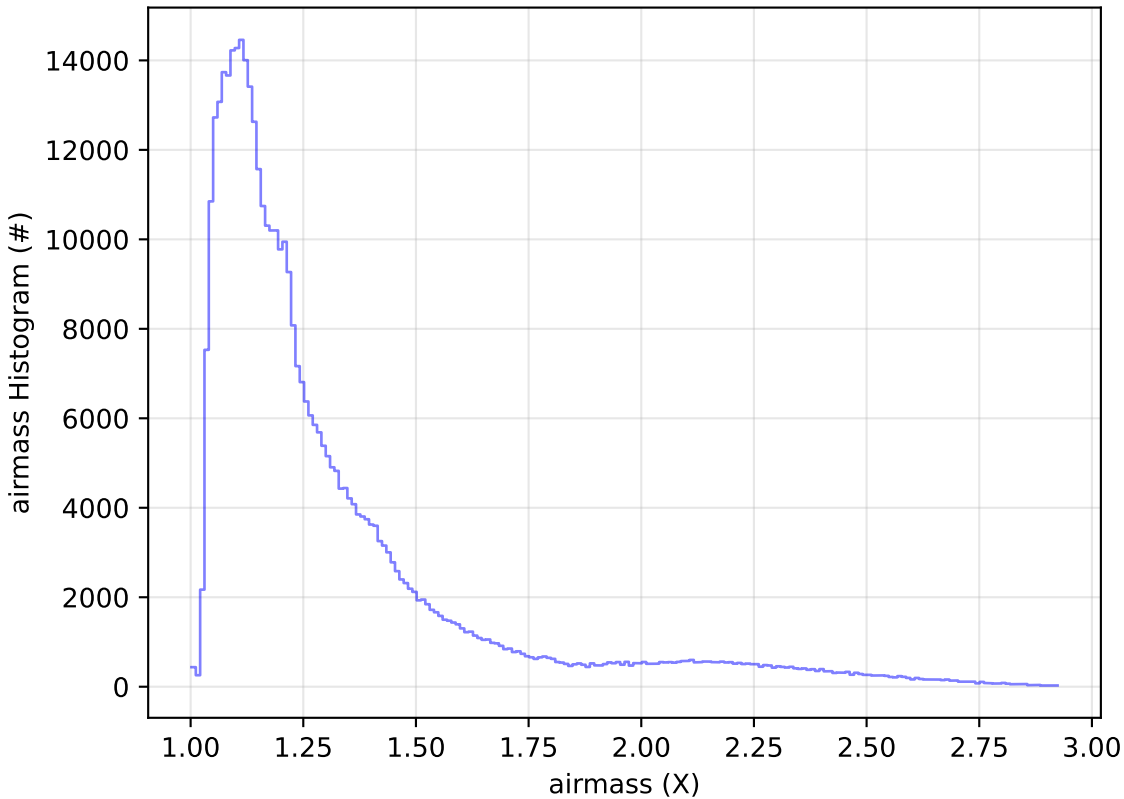
ddf_acor_sf30_lsf40_lsr10_v3.4_10yrs All sky z band: airmass Histogram
