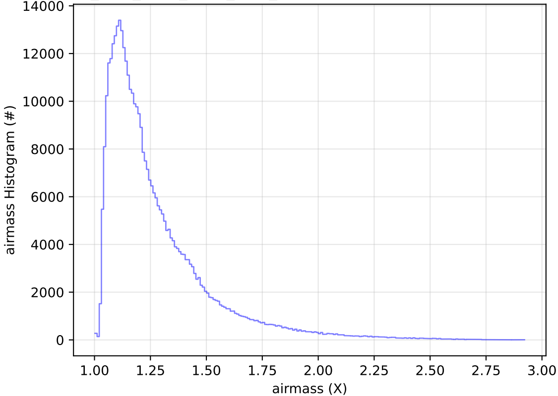
ddf_acor_sf30_lsf40_lsr10_v3.4_10yrs All sky y band: airmass Histogram
