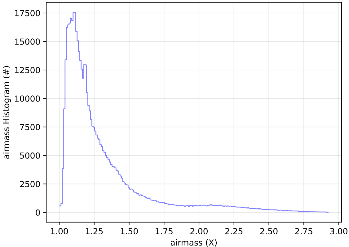
ddf_acor_sf30_lsf40_lsr10_v3.4_10yrs All sky i band: airmass Histogram
