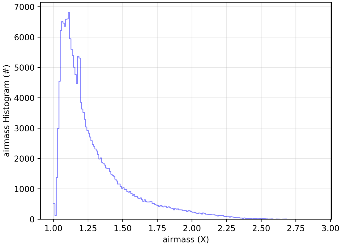
ddf_acor_sf30_lsf40_lsr10_v3.4_10yrs All sky g band: airmass Histogram
