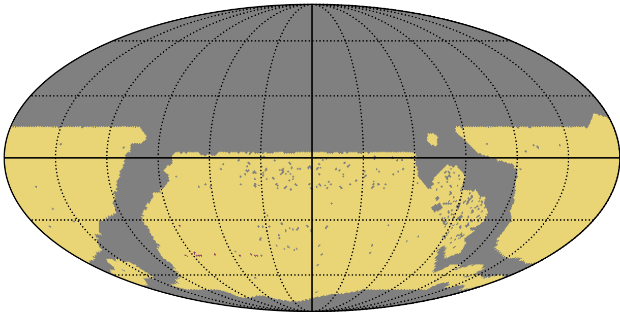
ddf_acor_sf30_lsf40_lsr10_v3.4_10yrs WFD: RapidRevisits
